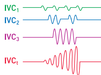
[ IVC single line diagram and the reactive power compensation current wave ]
